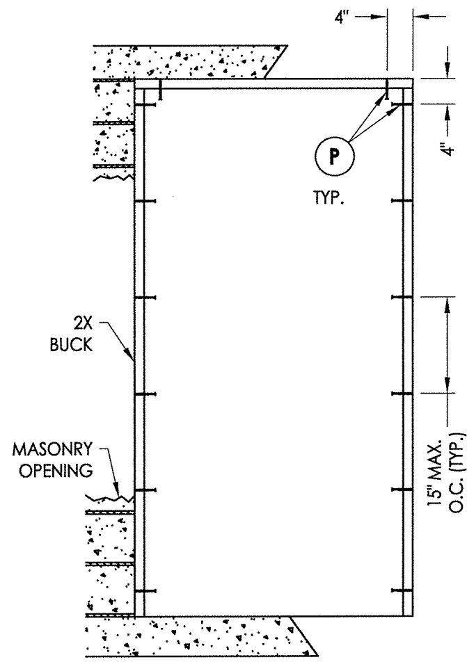
BUCK ANCHORING
