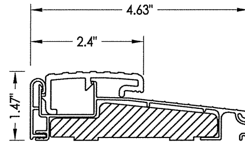
55 OUTSWING THRESHOLD
