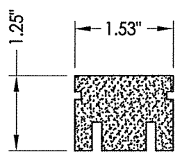
13 BOTTOM RAIL
