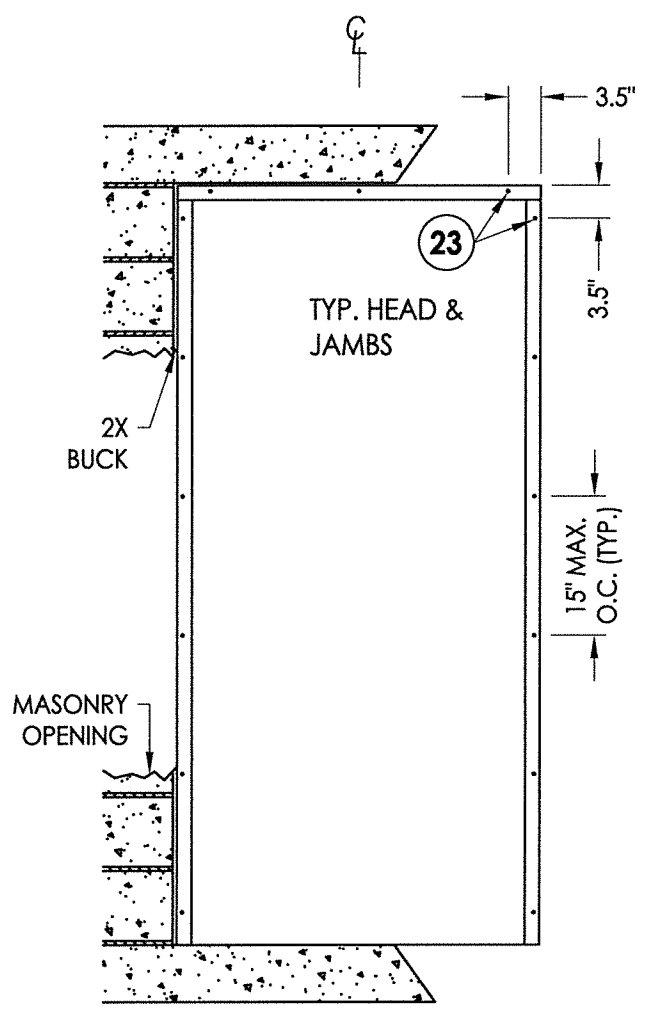
FRAME ANCHORING 2X MASONRY
