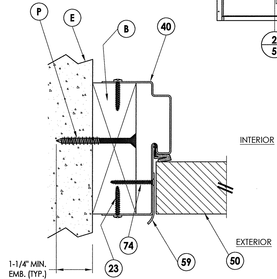
2 HORIZONTAL CROSS SECTION 4 2X wood buck @ latch Outswing shown (Inswing similar)
