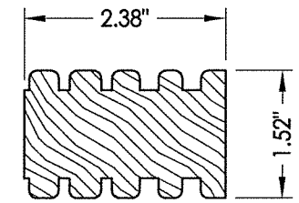
45 LOCK BLOCK
