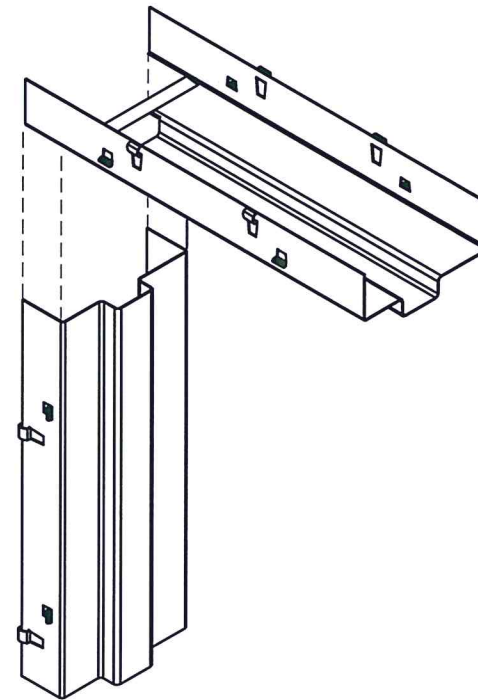
REDIFRAME ONE-PIECE
