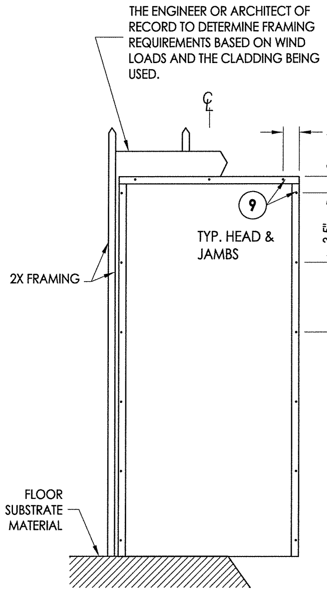
FRAME ANCHORING STUD CONSTRUCTION
