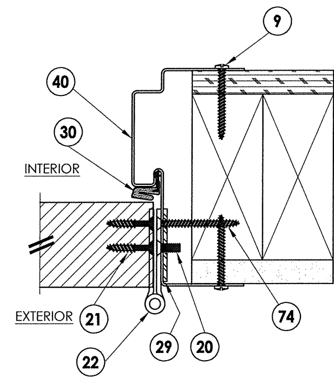
3 HORIZONTAL CROSS SECTION 4 Shown w/ stud construction Outswing shown (Inswing similar)
