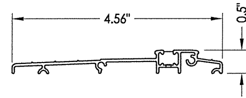
57 INSWING THRESHOLD
