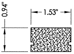
14 TOP RAIL
