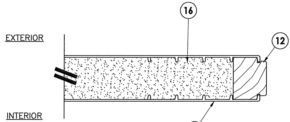
1 HORIZONTAL CROSS SECTION
